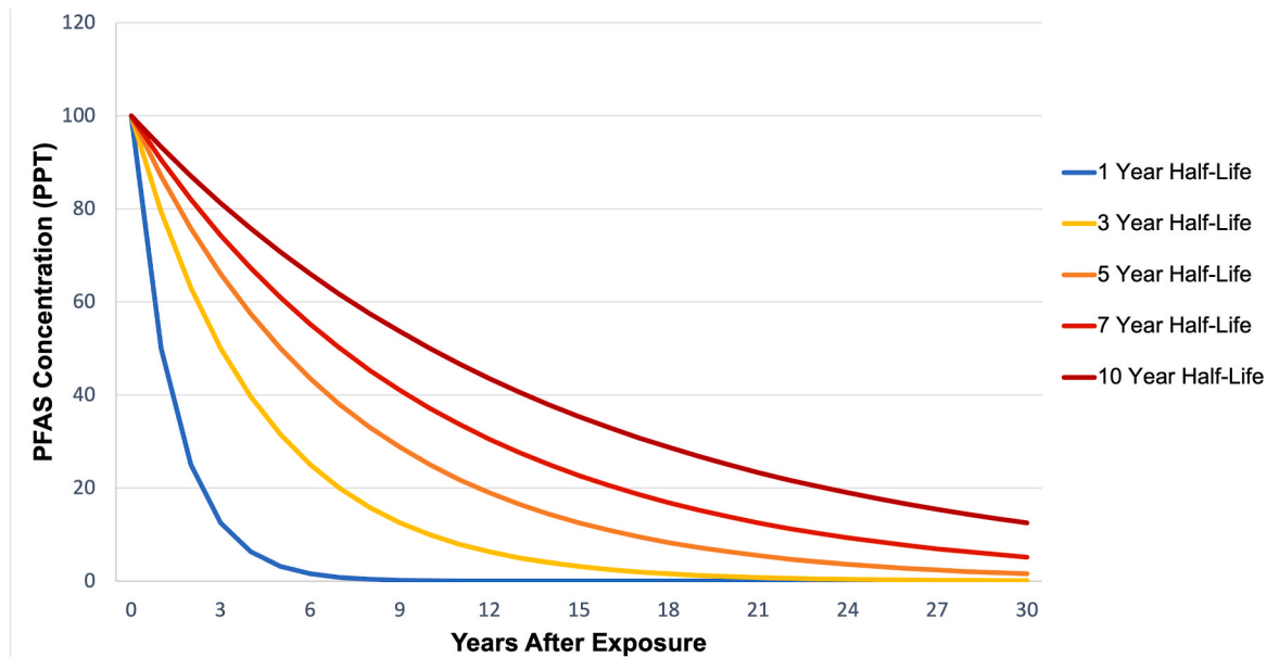
Fig. 2. Theoretical decay of PFAS chemicals in human blood serum with varying half-lives.
